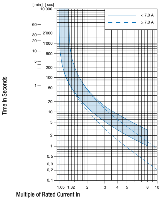
Multiple of Rated Current In Ambient temperature +23°
