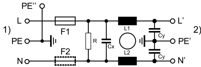
Standard Version with Bleed Resistor 1-1/2-pole
